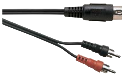
Standard 5 Pin DIN Plug to 2x Phono Plug Screened Lead
