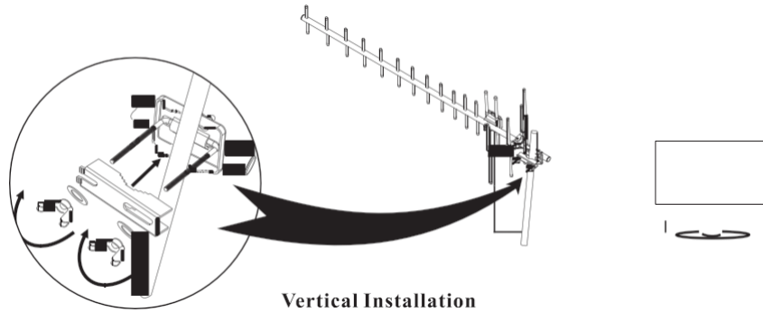
Vertical Installation
